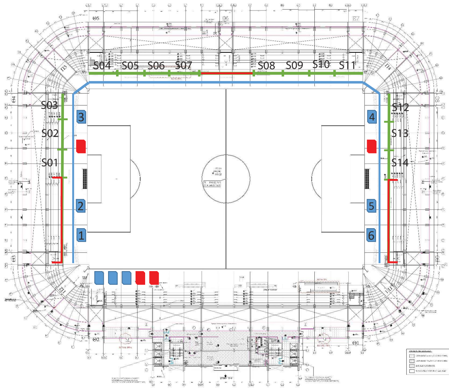
FIRST FLOOR SF 001.01 KATOPHT 1:100 (OP060) st. 1/200
